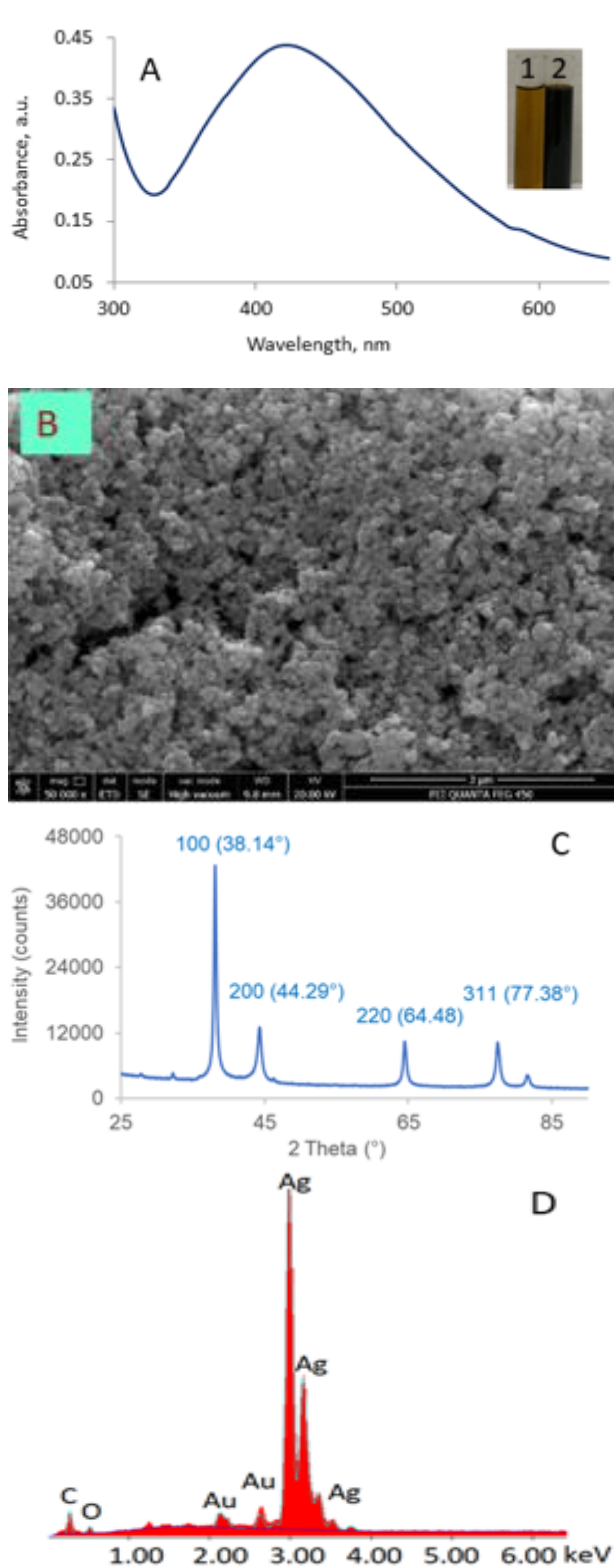
Figure 1. UV-Vis spectrum (A), extract solution (1) and AgNPs solution (2). SEM image (B). XRD spectrum (C). EDX spectrum (D).
