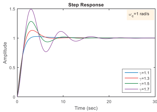
Figure 6: Unit-Step response with controller ( \omega_c=1 \text{ rad/s} )
