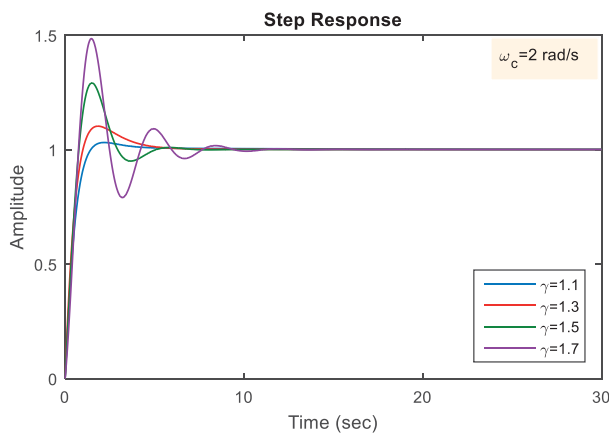
Figure 7: Unit-Step response with controller ( \omega_c=2 \text{ rad/s} )
