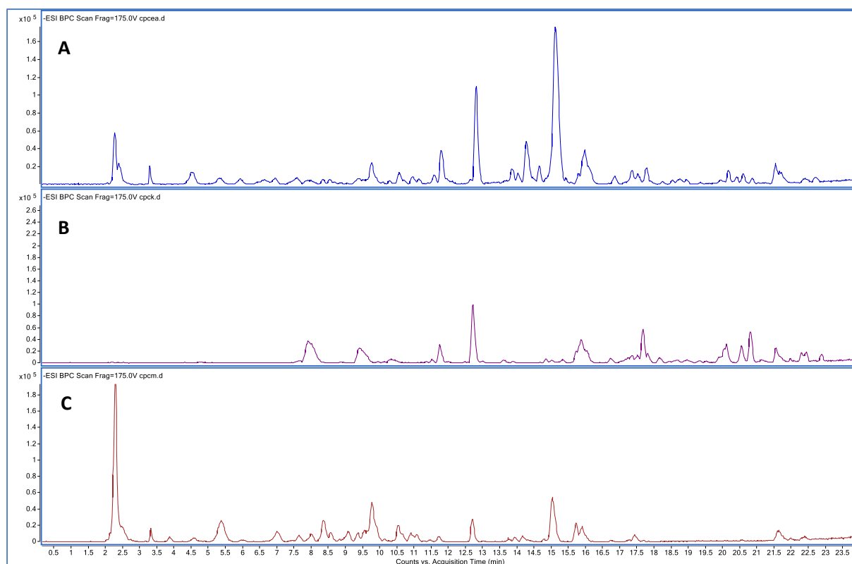
Figure 1. HPLC-TOF/MS chromatograms of CHCl 3 (A), EtOAc (B), and MeOH (C) extracts of CPP
