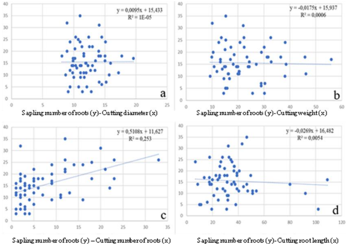
Figure 3. Relationships of mulberry sapling number of roots with initial cutting diameter (a), cutting weight (b), cutting number of roots (c) and cutting root length (d) values
