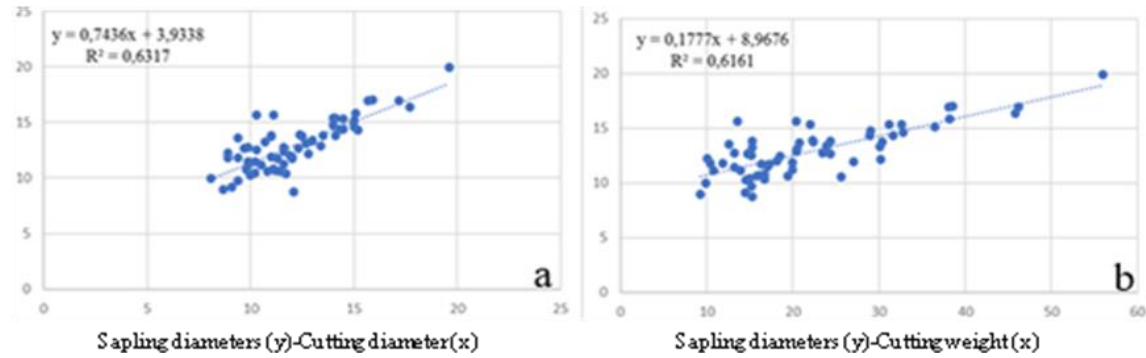
Figure 2. Relationships of black mulberry sapling diameters with initial cutting diameter (a), cutting weight (b)
