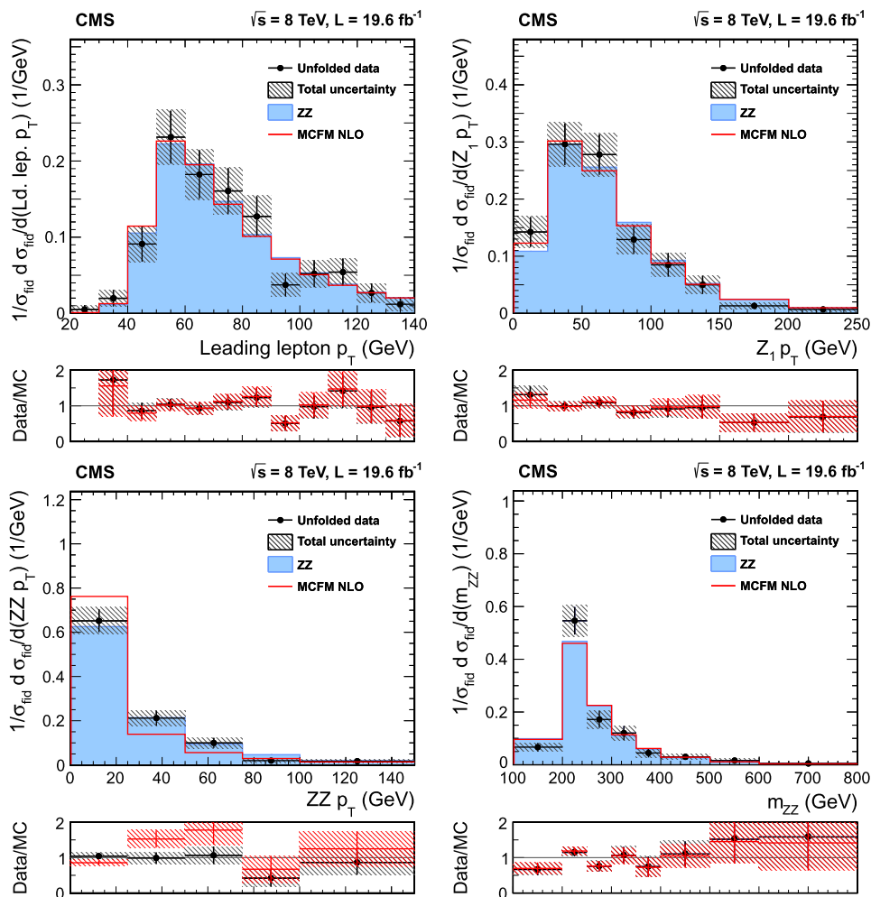
Fig. 3. Differential cross sections normalized to the fiducial cross section for the combined 4e , 4\mu , and 2e2\mu decay channels as a function of p_T for (upper left) the highest p_T lepton in the event, (upper right) the Z_1 , and (lower left) the ZZ system. Figure (lower right) shows the normalized d\sigma/dm_{ZZ} distribution. Points represent the data, and the shaded histograms labeled ZZ represent the POWHEG+GGZZ+PYTHIA predictions for ZZ signal, while the solid curves correspond to results of the MCFM calculations. The bottom part of each subfigure represents the ratio of the measured cross section to the expected one from POWHEG+GGZZ+PYTHIA (black crosses with solid symbols) and MCFM (red crosses). The shaded areas on all the plots represent the full uncertainties calculated as the quadrature sum of the statistical and systematic uncertainties, whereas the crosses represent the statistical uncertainties only. (For interpretation of the references to color in this figure legend, the reader is referred to the web version of this article.)
