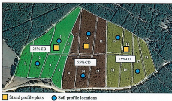
Figure 4: Location of stand profile plots and soil profile locations at the three canopy densities (CD)
